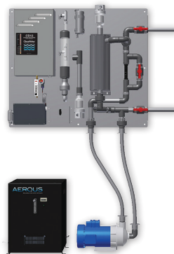
CIP 800 Panel-Mounted
