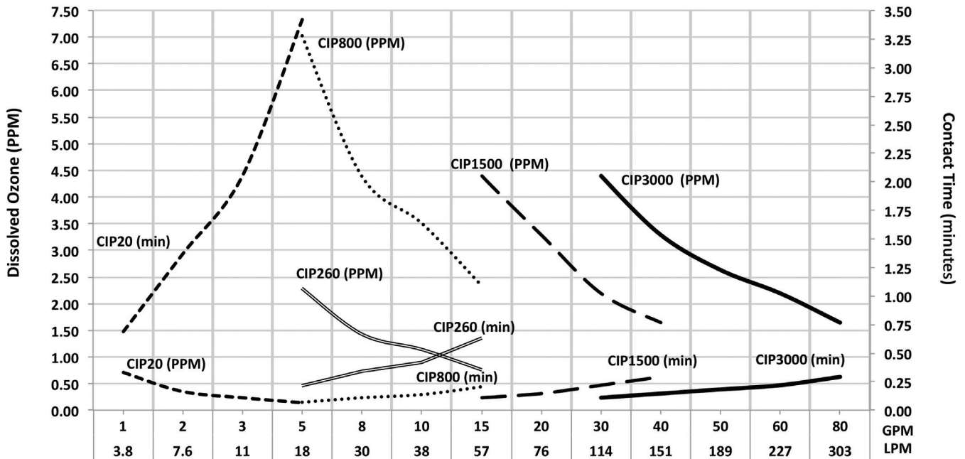
CIP - Series Dissolved Ozone and Contact Time
